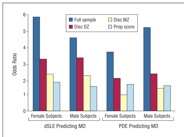
Figure 2. The odds ratio for the prediction of an episode of major depression (MD) as predicted by the occurrence of a dependent stressful life event (dSLE) or a prior depressive episode (PDE) in the full twin sample, in monozygotic twins discordant for the risk factor exposure (Disc MZ), in dizygotic twins discordant for the risk factor exposure (Disc DZ), and in simulated case-control pairs matched on propensity scores (Prop score). These results are presented separately in male and female twins.
