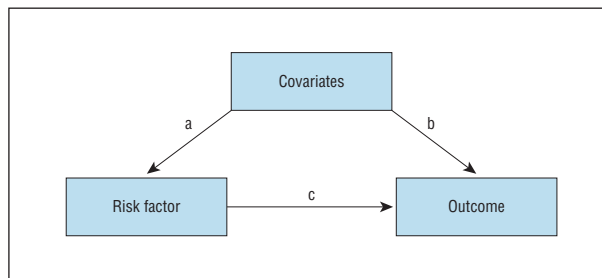
Figure 1. The interrelationship among a risk factor, a potential covariate, and an outcome. The causal interrelationship between the risk factor and the outcome is depicted by path c, whereas the noncausal pathway is captured by paths a and b.
