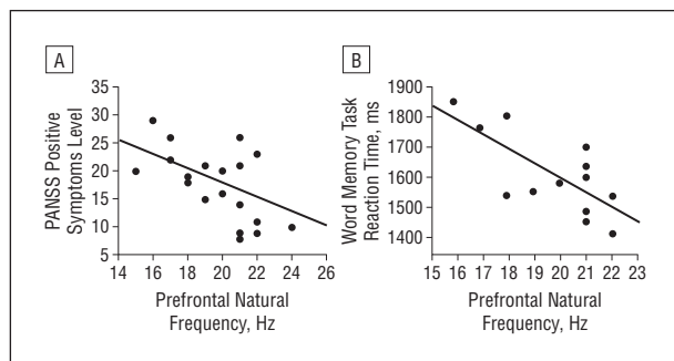
Figure 3. The frequency of prefrontal cortex oscillations was inversely related to the level of positive symptoms on the Positive and Negative Syndrome Scale (PANSS) (A) as well as to the reaction time of correct responses on a word memory task (B) in patients with schizophrenia.
