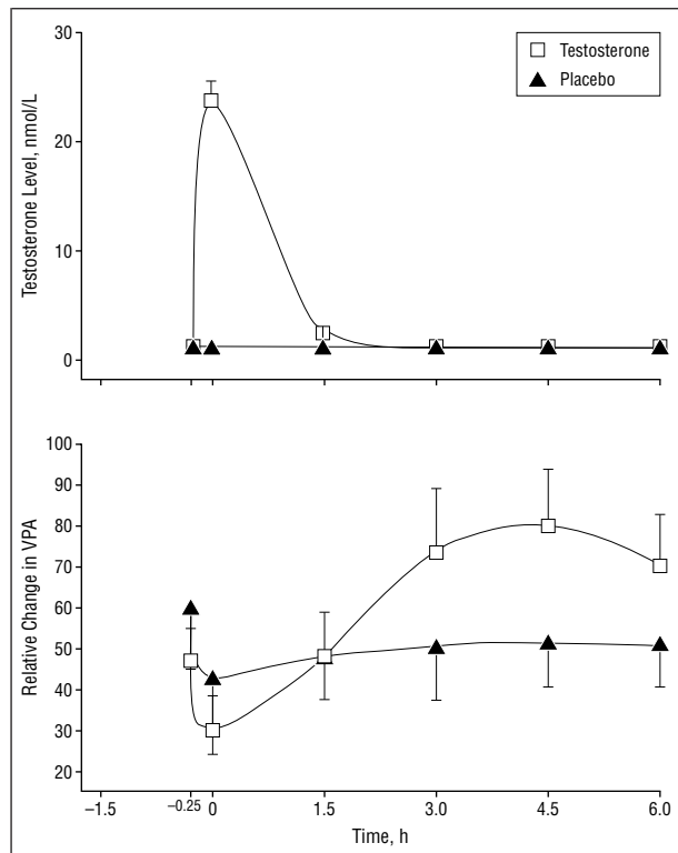
Figure 1. Top, Average levels of total testosterone at different times during placebo and testosterone undecanoate treatment ( N = 8 ). To convert testosterone from nanomoles per liter to nanograms per deciliter, divide nanomoles per liter by 0.0347. Bottom, Average relative increases in vaginal pulse amplitude (VPA) induced by erotic film excerpts viewed at 6 consecutive times during placebo and testosterone treatment ( N = 8 ). Error bars indicate SEM.
